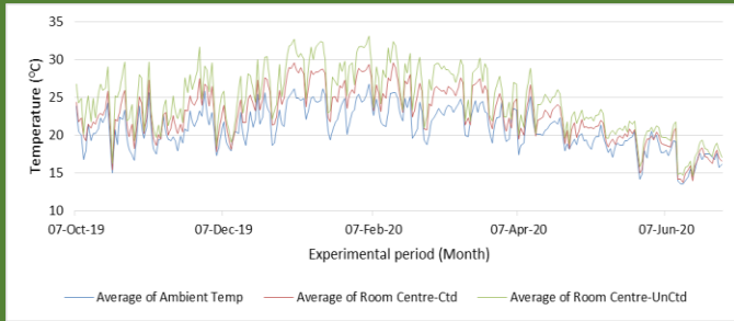
Figure 11: Daily average temperature of ambient, coated and uncoated air temperatures
